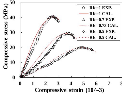
Fig. 14. Comparison between experimental and analytical compressive stress-strain curves
