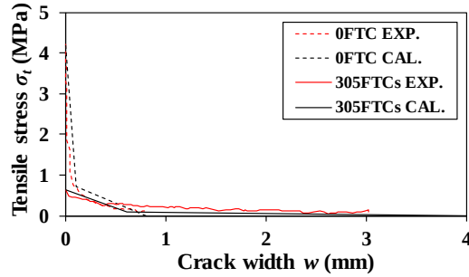
Fig. 16. Comparison between experimental and analytical tension softening curves
