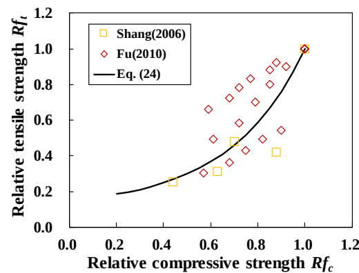
Fig. 12. Comparison of Rf_t between proposed model and experiments
