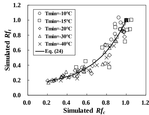
Fig. 11. Relationships between Rf_t versus Rf_c by RBSM simulation
