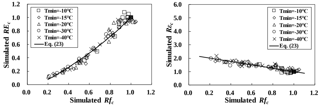
Fig. 8. Relationships between (a) RE_c and (b) RE_c versus Rf_c by RBSM simulation
