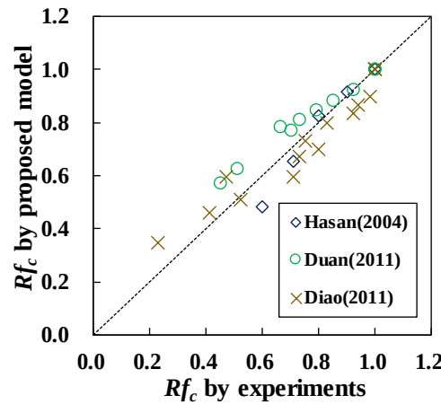
Fig. 7. Comparison of relative compressive strength by proposed model and experiments
