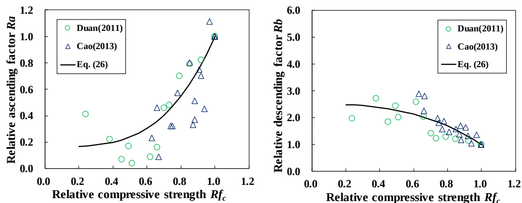
Fig. 13. Relationships between relative compressive strength and (a) Ra_d (b) Rb_d
