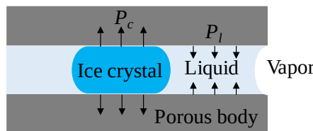
Fig. 2. Cryosuction and crystallization pressure in a cylindrical pore
