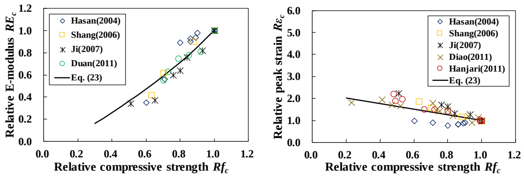
Fig. 9. Comparisons of (a) RE_c and (b) RE_c between proposed models and experiments
